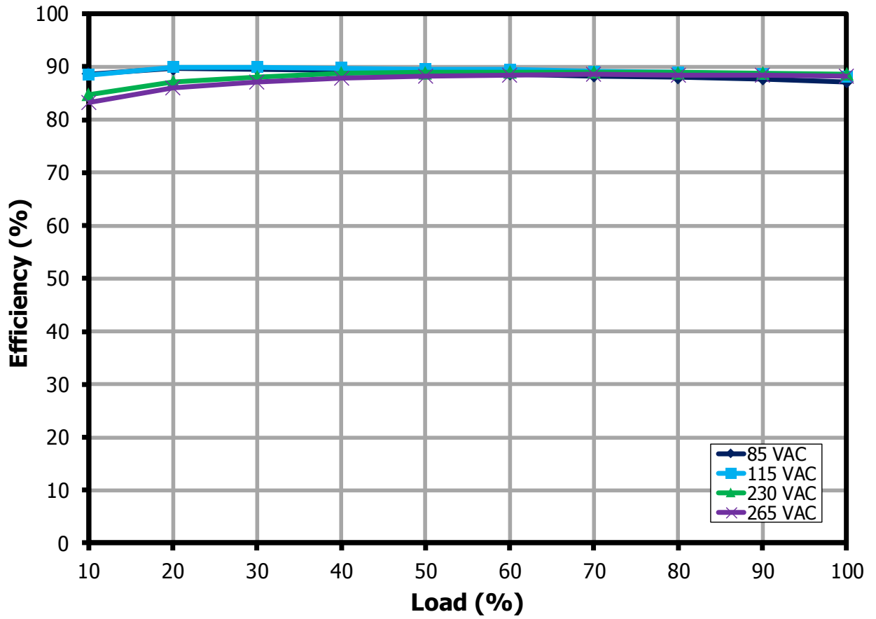
Figure 20 – 5 V Efficiency Across Load.
