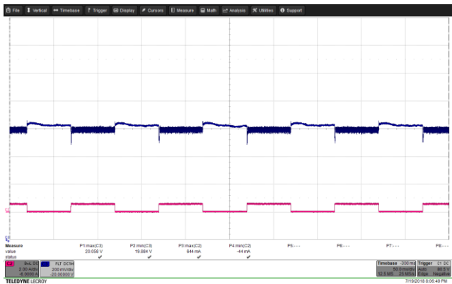
Figure 72 – Transient Response. 85 VAC, 20.0 V, 0 – 0.56 A Load Step. V_{MIN} 19.884 V, V_{MAX} : 20.058 V. Upper: V_{OUT} , 0.2 V / div., 50 ms / div. Lower: I_{LOAD} , 2 A / div.
