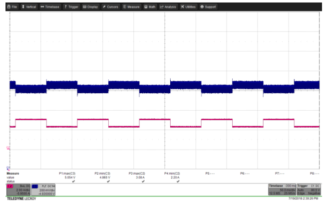
Figure 55 – Transient Response. 265 VAC, 5.0 V, 2.25 – 3 A Load Step. V_{MIN} : 4.865 V, V_{MAX} : 5.054 V. Upper: V_{OUT} , .2 V / div., 50 ms / div. Lower: I_{LOAD} , 2 A / div.
