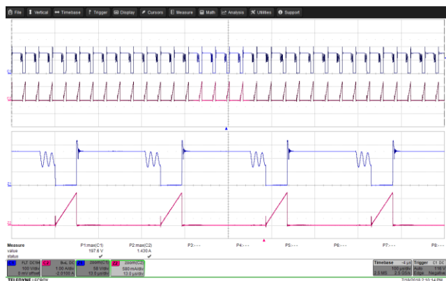
Figure 80 – Drain Voltage and Current Waveforms. 85 VAC, 5.0 V, 3 A Load (197.6 V MAX ). Upper: V DRAIN , 100 V, 100 μs / div. Lower: I DRAIN , 1 A / div.
