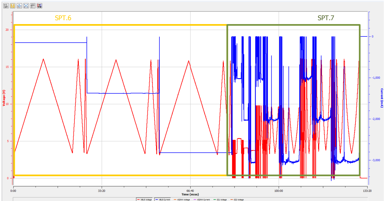
Figure 109 – Plot of SPT.6 VST Test and SPT.7 CLT Test from Total Phase Analyzer.
