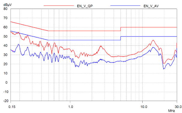
Figure 115 – Floating Ground EMI, 11 V / 2.45 A Load [Line Scan].
