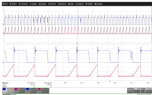
Figure 82 – Drain Voltage and Current Waveforms. 85 VAC, 9.0 V, 3 A Load (217.5 V MAX ). Upper: V DRAIN , 100 V, 100 μs / div. Lower: I DRAIN , 1 A / div.
