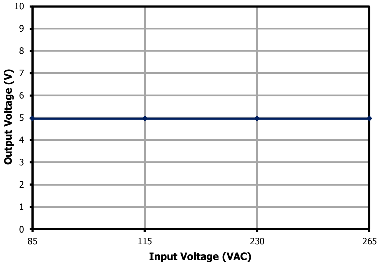
Figure 24 – Output Voltage vs. Input Line Voltage for 5 V Output, Room Temperature.
