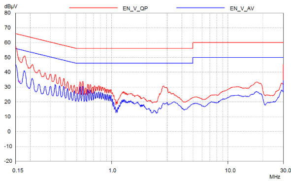
Figure 112 – Floating Ground EMI, 5 V / 3 A Load [Line Scan].
