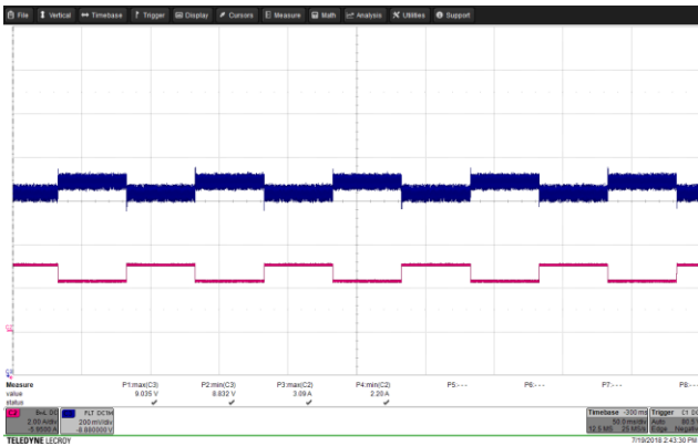
Figure 62 – Transient Response. 85 VAC, 9.0V, 2.25 – 3 A Load Step. V_{MIN} : 8.832 V, V_{MAX} : 9.035 V. Upper: V_{OUT} , .2 V / div., 50 ms / div. Lower: I_{LOAD} , 2 A / div.
