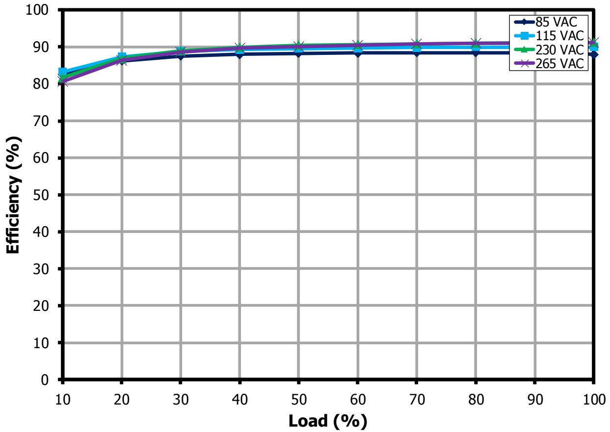
Figure 23 – 20 V Efficiency Across Load.
