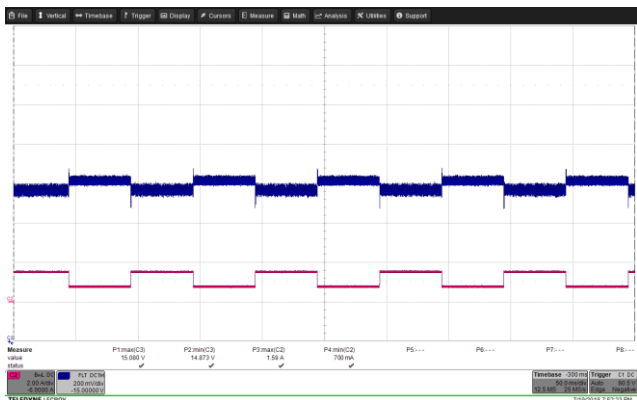
Figure 66 – Transient Response. 85 VAC, 15.0 V, 0.75 – 1.5 A Load Step. V_{MIN} 14.873 V, V_{MAX} : 15.080 V. Upper: V_{OUT} , 0.2 V / div., 50 ms / div. Lower: I_{LOAD} , 2 A / div.
