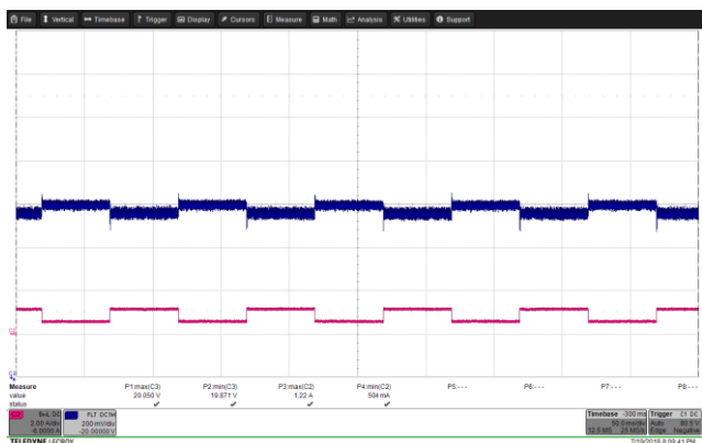
Figure 74 – Transient Response. 85 VAC, 20.0 V, 0.56 – 1.125 A Load Step. V_{MIN} 19.871 V, V_{MAX} : 20.050 V. Upper: V_{OUT} , 0.2 V / div., 50 ms / div. Lower: I_{LOAD} , 2 A / div.
