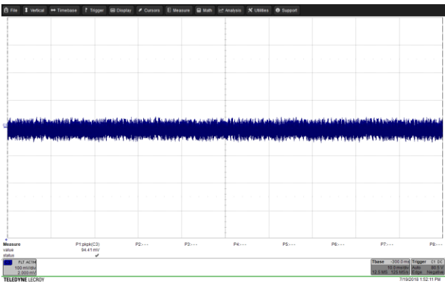
Figure 102 – Output Ripple. PK-PK = 94.41 mV. 85 VAC IN 9.0 V, 3 A Load. V OUT , 100 mV / div., 10 ms / div.
