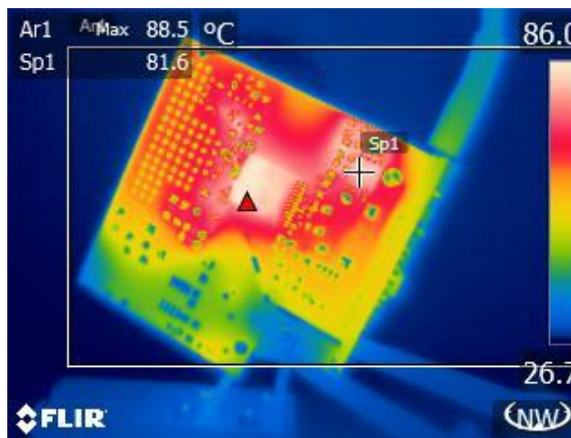
Figure 43 – InnoSwitch3-Pro Side. Ambient = 27.3 °C. InnoSwitch3-Pro = 88.5 °C. SR FET, Q2 = 81.6 °C.
