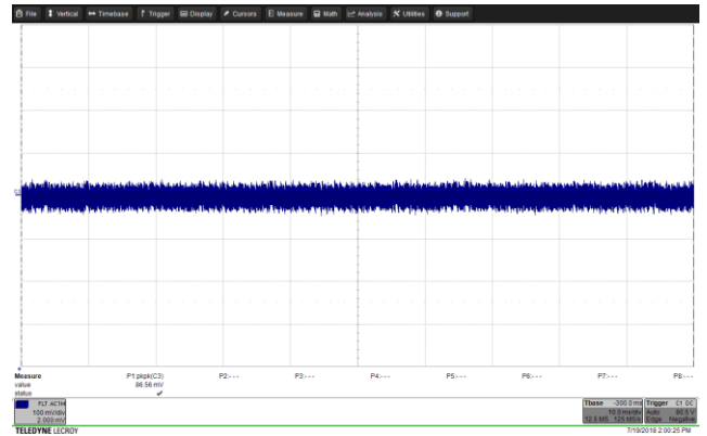
Figure 105 – Output Ripple. PK-PK = 86.56 mV. 265 VAC IN 15.0 V, 3 A Load. V OUT , 100 mV / div., 10 ms / div.
