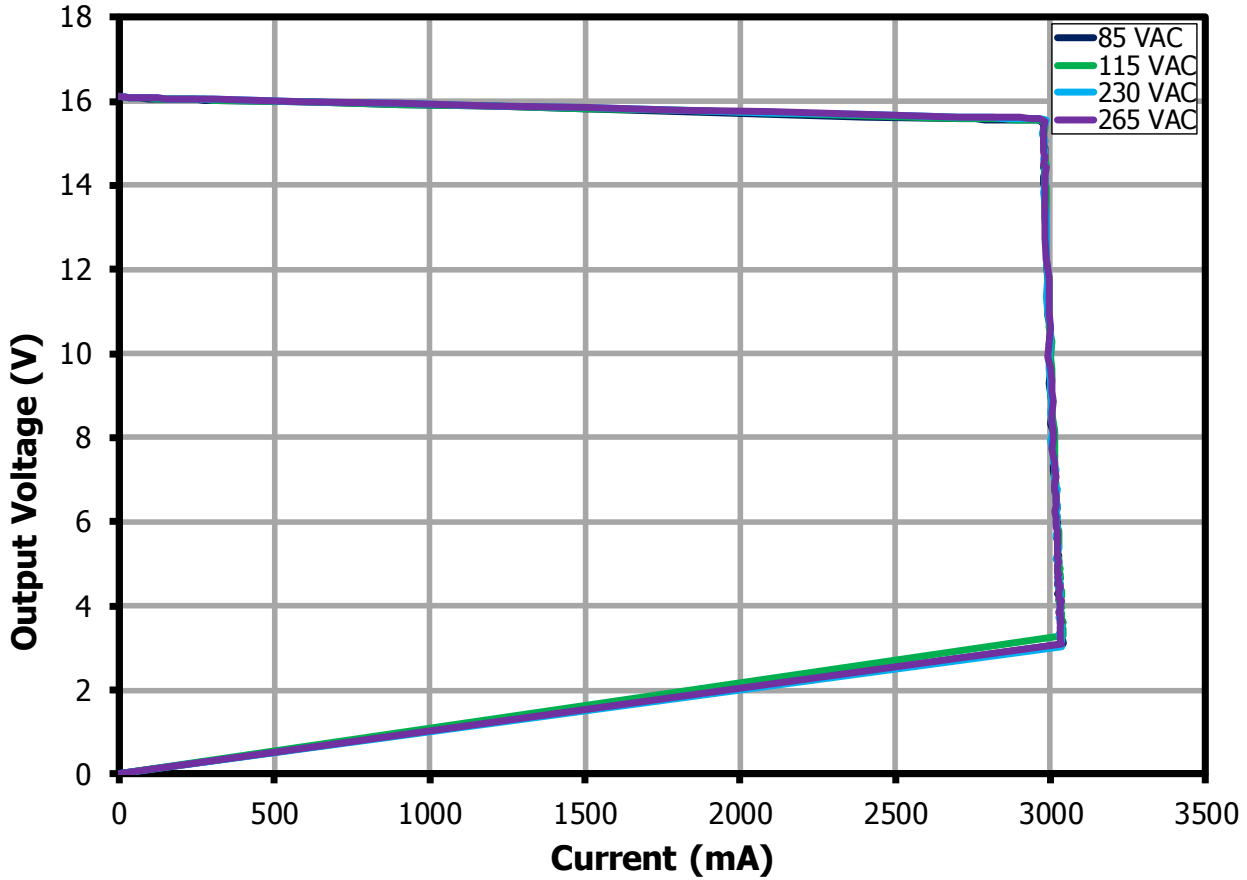
Figure 108 – CV/CC Profile with output 16 V, 3 A.
