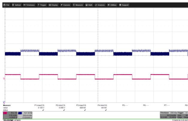
Figure 49 – Transient Response. 265 VAC, 5.0 V, 0 – 0.75 A Load Step. V_{MIN} 5.006 V, V_{MAX} : 5.128 V. Upper: V_{OUT} , 0.2 V / div., 50 ms / div. Lower: I_{LOAD} , 2 A / div.
