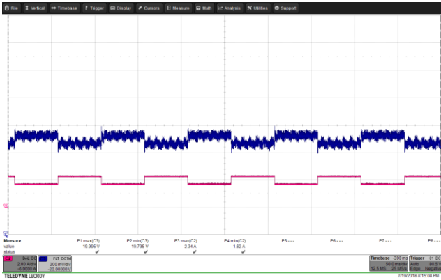
Figure 78 – Transient Response. 85 VAC, 20.0V, 1.68 – 2.25 A Load Step. V_{MIN} : 19.795 V, V_{MAX} : 19.995 V. Upper: V_{OUT} , .2 V / div., 50 ms / div. Lower: I_{LOAD} , 2 A / div.
