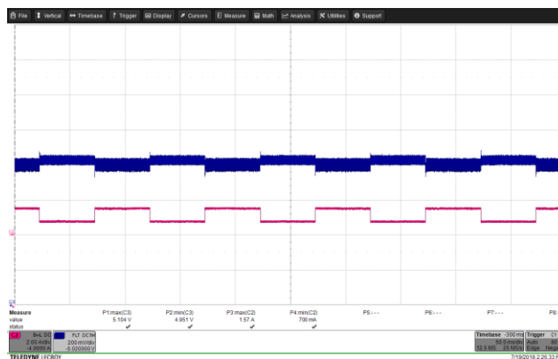
Figure 51 – Transient Response. 265 VAC, 5.0 V, 0.75 – 1.5 A Load Step. V_{MIN} 4.951 V, V_{MAX} : 5.104 V. Upper: V_{OUT} , 0.2 V / div., 50 ms / div. Lower: I_{LOAD} , 2 A / div.
