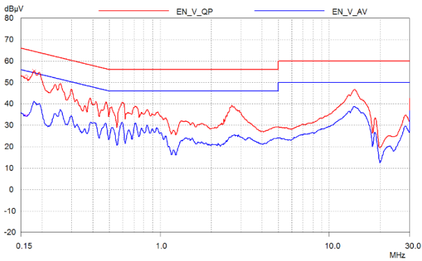
Figure 114 – Floating Ground EMI, 3 V / 3 A Load [Line Scan].
