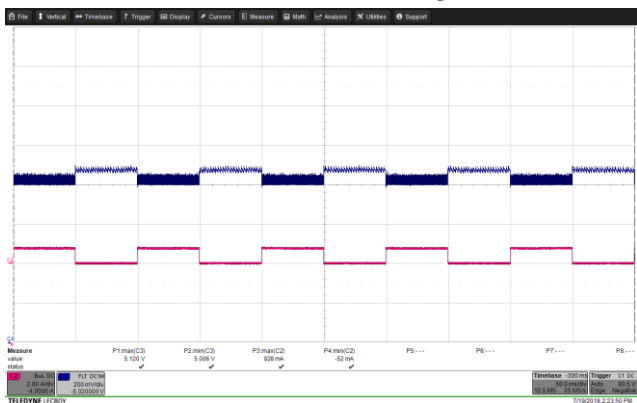
Figure 48 – Transient Response. 85 VAC, 5.0 V, 0 – 0.75 A Load Step. V_{MIN} 5.006 V, V_{MAX} : 5.120 V. Upper: V_{OUT} , 0.2 V / div., 50 ms / div. Lower: I_{LOAD} , 2 A / div.
