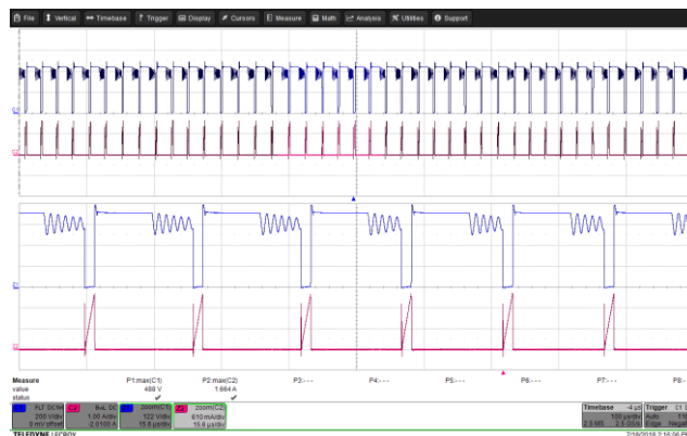
Figure 83 – Drain Voltage and Current Waveforms. 265 VAC, 9 V, 3 A Load (488 V MAX ). Upper: V DRAIN , 200 V, 100 μs / div. Lower: I DRAIN , 1 A / div.
