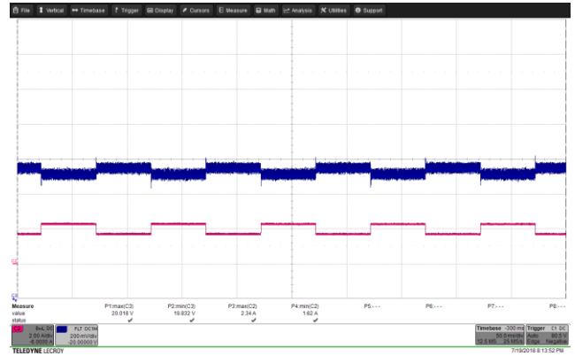
Figure 79 – Transient Response. 265VAC, 20.0V, 1.68 – 2.25 A Load Step. V_{MIN} : 19.832 V, V_{MAX} : 20.018 V. Upper: V_{OUT} , .2 V / div., 50 ms / div. Lower: I_{LOAD} , 2 A / div.
