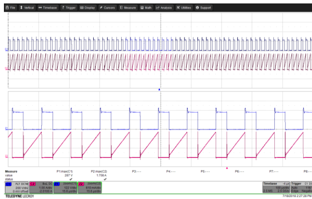
Figure 86 – Drain Voltage and Current Waveforms. 85 VAC, 20.0 V, 2.25 A Load (287 V_{MAX} ). Upper: V_{DRAIN} , 200 V, 100 \mu s / div. Lower: I_{DRAIN} , 1 A / div.
