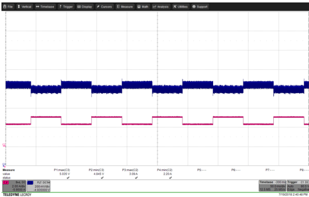
Figure 54 – Transient Response. 85 VAC, 5.0 V, 2.25 – 3 A Load Step. V_{MIN} : 4.845 V, V_{MAX} : 5.035 V. Upper: V_{OUT} , .2 V / div., 50 ms / div. Lower: I_{LOAD} , 2 A / div.
