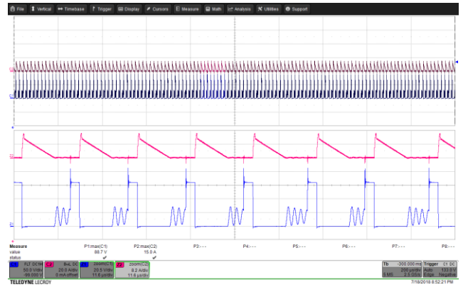
Figure 93 – SR FET Voltage Waveforms. 265 VAC, 15.0 V, 3 A Load (88.7 V MAX ). Upper: V DRAIN , 50 V, 200 μs / div. Lower: I DRAIN , 10 A / div.
