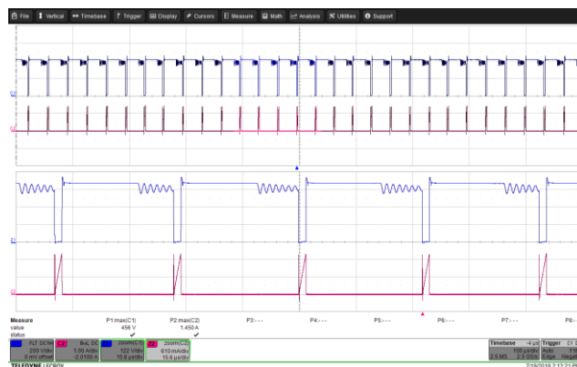
Figure 81 – Drain Voltage and Current Waveforms. 265 VAC, 5.0 V, 3 A Load (456 V MAX ). Upper: V DRAIN , 200 V, 100 μs / div. Lower: I DRAIN , 1 A / div.
