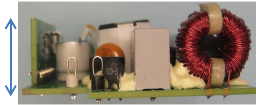
Figure 4 – Populated Circuit Board Photograph (Side View)
