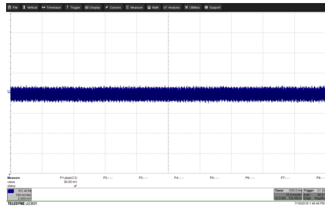
Figure 103 – Output Ripple. PK-PK = 90.85 mV. 265 VAC IN 9.0 V, 3 A Load. V OUT , 100 mV / div., 10 ms / div.
