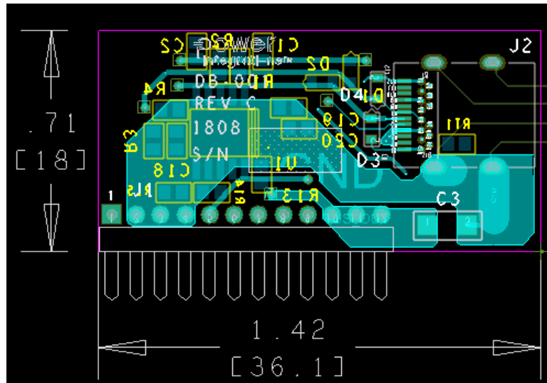
Figure 10 – Printed Circuit Layout, Daughter Board, Top.
