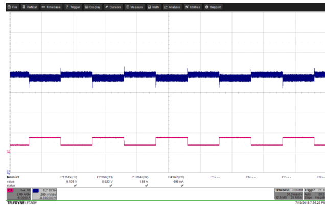
Figure 59 – Transient Response. 265 VAC, 9.0 V, 0.75 – 1.5 A Load Step. V_{MIN} 8.923 V, V_{MAX} : 9.136 V. Upper: V_{OUT} , 0.2 V / div., 50 ms / div. Lower: I_{LOAD} , 2 A / div.
