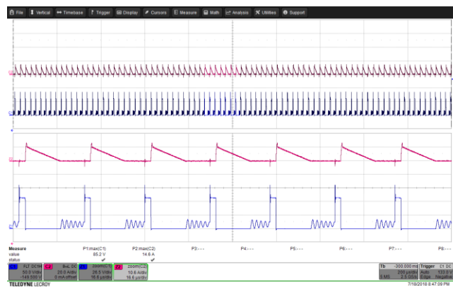
Figure 91 – SR FET Voltage Waveforms. 265 VAC, 9.0 V, 3 A Load (85.2 V_{MAX} ). Upper: V_{DRAIN} , 50 V, 200 \mu s / div. Lower: I_{DRAIN} , 10 A / div.
