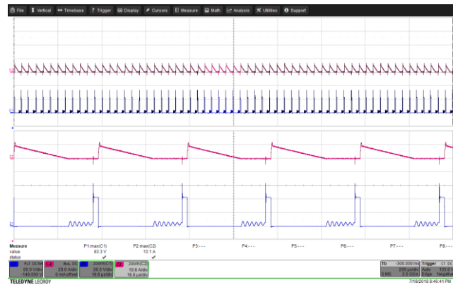
Figure 89 – SR FET Voltage Waveforms. 265 VAC, 5.0 V, 3 A Load (83.3 V_{MAX} ). Upper: V_{DRAIN} , 50 V, 200 \mu s / div. Lower: I_{DRAIN} , 10 A / div.
