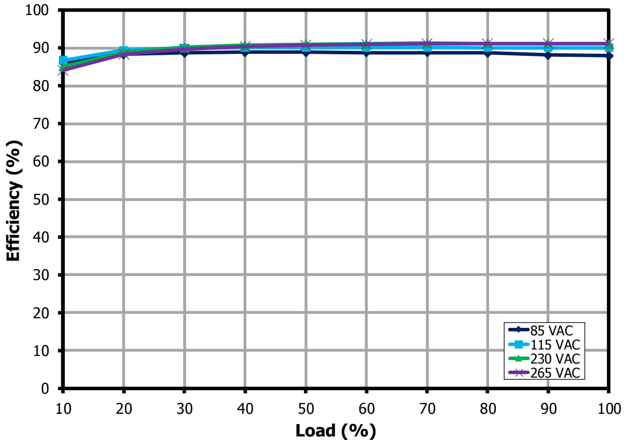
Figure 22 – 15 V Efficiency Across Load.
