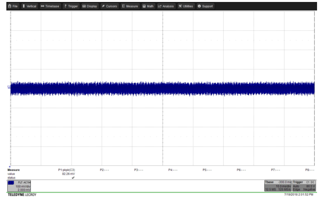
Figure 107 – Output Ripple. PK-PK = 82.26 mV. 265 VAC IN 20.0 V, 2.25 A Load. V OUT , 100 mV / div., 10 ms / div.
