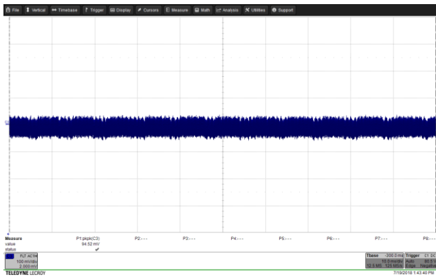
Figure 100 – Output Ripple. PK-PK = 94.52 mV. 85 VAC IN 5.0 V, 3 A Load. V OUT , 100 mV / div., 10 ms / div.
