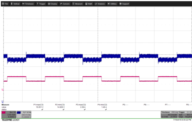
Figure 68 – Transient Response. 85 VAC, 15 V, 1.5 – 2.25 A Load Step. V_{MIN} : 14.828 V, V_{MAX} : 15.051 V. Upper: V_{OUT} , 0.2 V / div., 50 ms / div. Lower: I_{LOAD} , 2 A / div.
