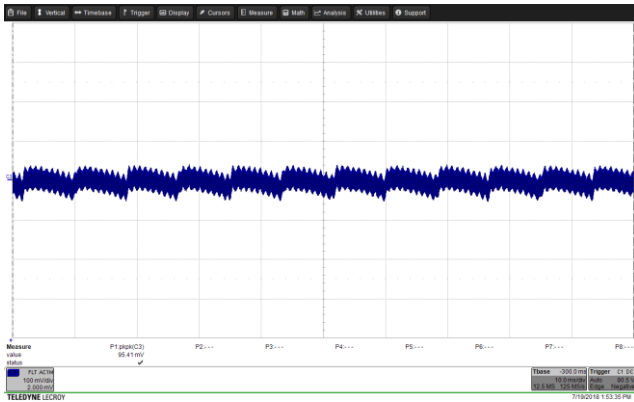
Figure 104 – Output Ripple. PK-PK = 95.41 mV. 85 VAC IN , 15.0 V, 3 A Load. V OUT , 100 mV / div., 10 ms / div.
