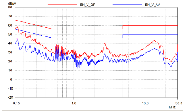
Figure 113 – Floating Ground EMI, 9 V / 3 A Load [Line Scan].
