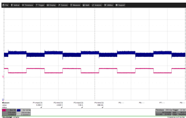
Figure 50 – Transient Response. 85 VAC, 5.0 V, 0.75 – 1.5 A Load Step. V_{MIN} 4.928 V, V_{MAX} : 5.099 V. Upper: V_{OUT} , 0.2 V / div., 50 ms / div. Lower: I_{LOAD} , 2 A / div.
