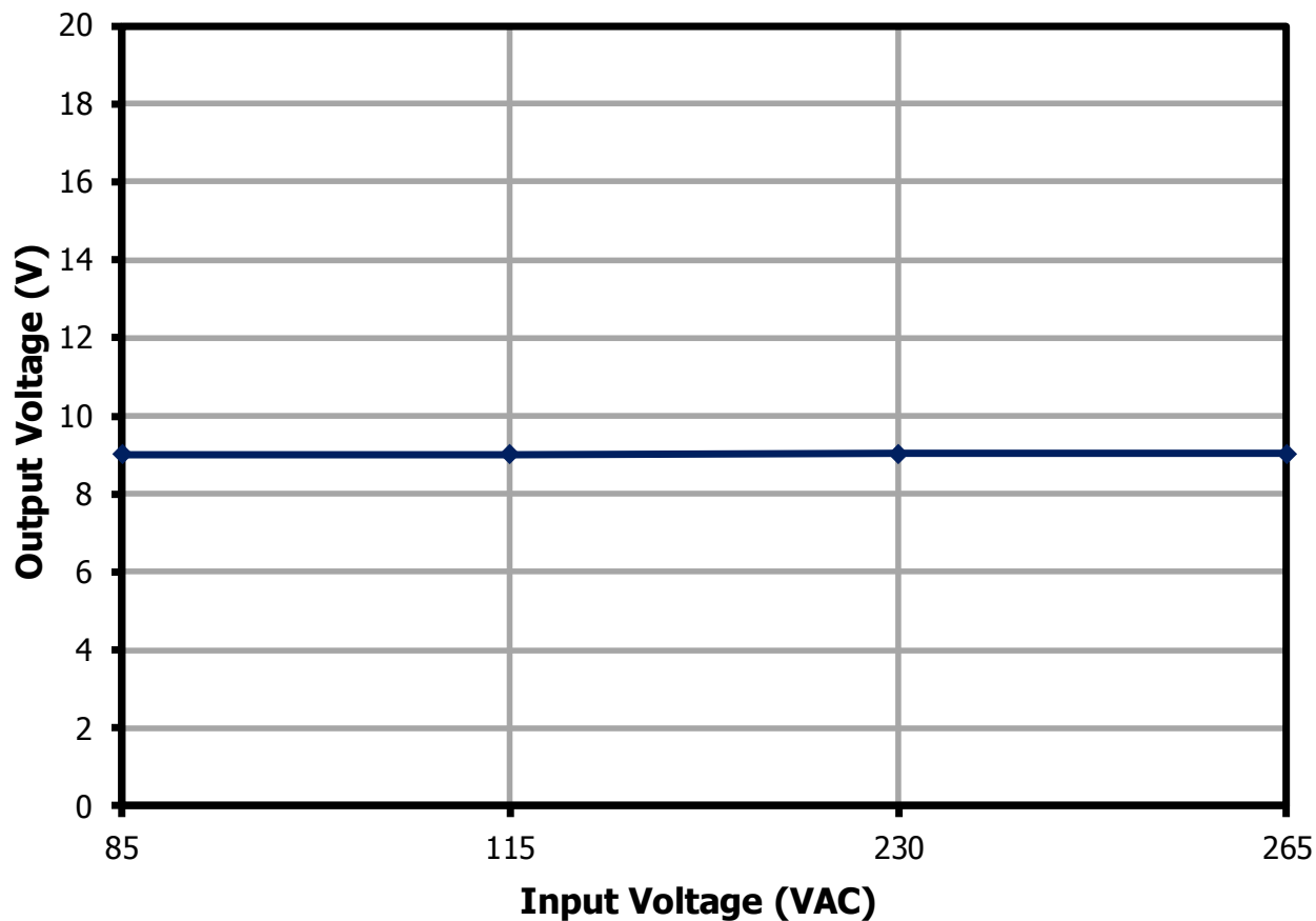
Figure 25 – Output Voltage vs. Input Line Voltage for 9 V Output, Room Temperature.
