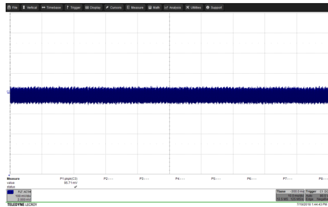
Figure 101 – Output Ripple. PK-PK = 95.71 mV. 265 VAC IN 5.0 V, 3 A Load. V OUT , 100 mV / div., 10 ms / div.
