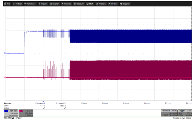
Figure 97 – Drain Voltage and Current Waveforms. 265 VAC, 5.0 V, 3 A Load (414.0 V_{MAX} ). Upper: V_{DRAIN} , 200 V, 100 ms / div. Lower: I_{DRAIN} , 1 A / div.
