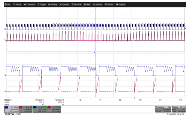
Figure 87 – Drain Voltage and Current Waveforms. 265 VAC, 20 V, 2.25 A Load (557 V_{MAX} ). Upper: V_{DRAIN} , 500 V, 100 \mu s / div. Lower: I_{DRAIN} , 1 A / div.
