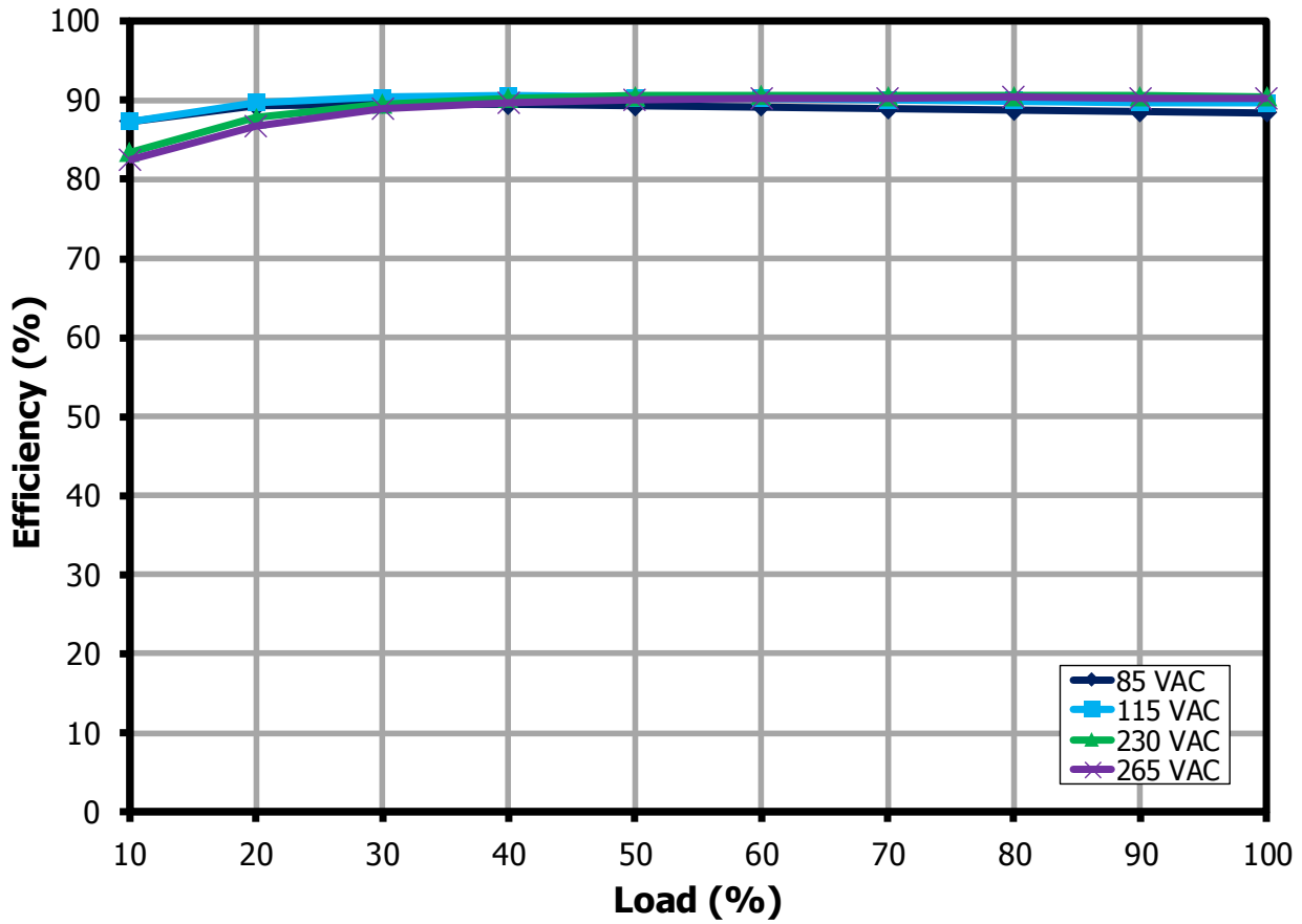
Figure 21 – 9 V Efficiency Across Load.
