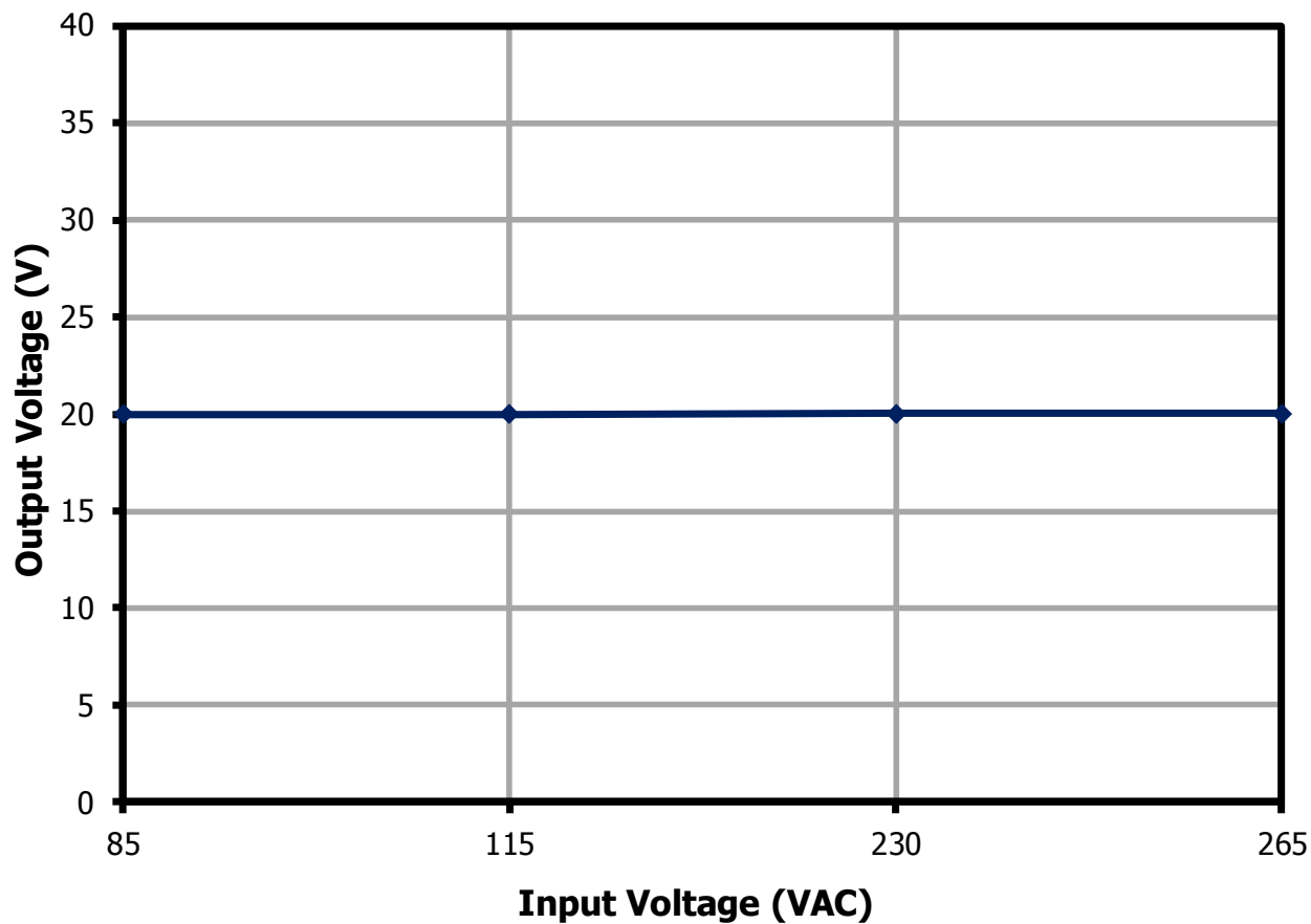
Figure 27 – Output Voltage vs. Input Line Voltage for 20 V Output, Room Temperature.
