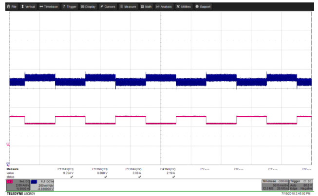
Figure 63 – Transient Response. 265 VAC, 9.0 V, 2.25 – 3 A Load Step. V_{MIN} : 8.868 V, V_{MAX} : 9.054 V. Upper: V_{OUT} , .2 V / div., 50 ms / div. Lower: I_{LOAD} , 2 A / div.
