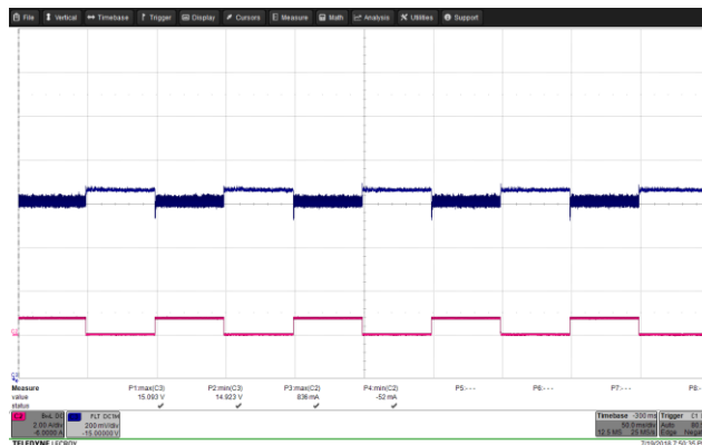
Figure 65 – Transient Response. 265 VAC, 15.0 V, 0 – 0.75 A Load Step. V_{MIN} 14.923 V, V_{MAX} : 15.093 V. Upper: V_{OUT} , 0.2 V / div., 50 ms / div. Lower: I_{LOAD} , 2 A / div.
