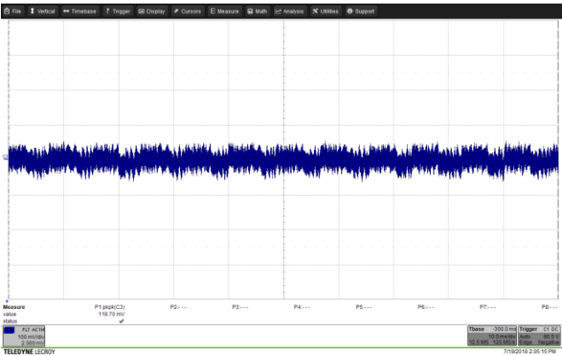
Figure 106 – Output Ripple. PK-PK = 118.70 mV. 85 VAC IN , 20.0 V, 2.25 A Load. V OUT , 100 mV / div., 10 ms / div.
