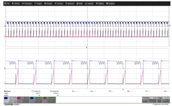
Figure 85 – Drain Voltage and Current Waveforms. 265 VAC, 15 V, 3 A Load (528 V_{MAX} ). Upper: V_{DRAIN} , 500 V, 100 \mu s / div. Lower: I_{DRAIN} , 1 A / div.
