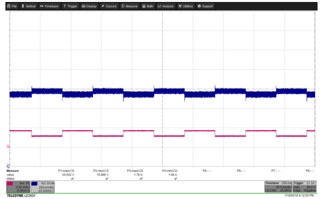
Figure 77 – Transient Response. 265 VAC, 20.0 V, 1.125 – 1.68 A Load Step. V_{MIN} : 19.866 V, V_{MAX} : 20.042 V. Upper: V_{OUT} , 0.2 V / div., 50 ms / div. Lower: I_{LOAD} , 2 A / div.
