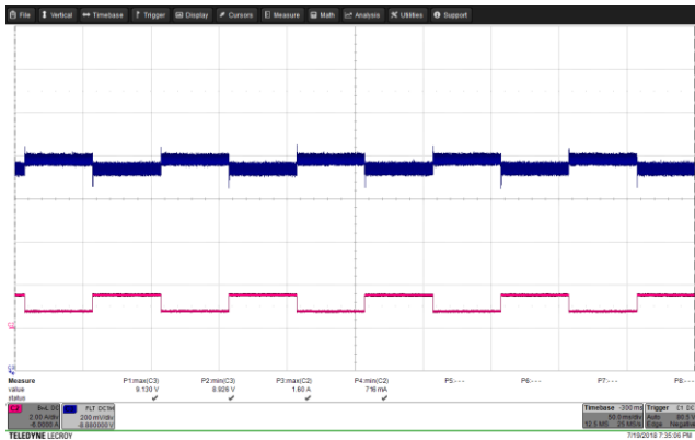
Figure 58 – Transient Response. 85 VAC, 9.0 V, 0.75 – 1.5 A Load Step. V_{MIN} 8.926 V, V_{MAX} : 9.130 V. Upper: V_{OUT} , 0.2 V / div., 50 ms / div. Lower: I_{LOAD} , 2 A / div.
