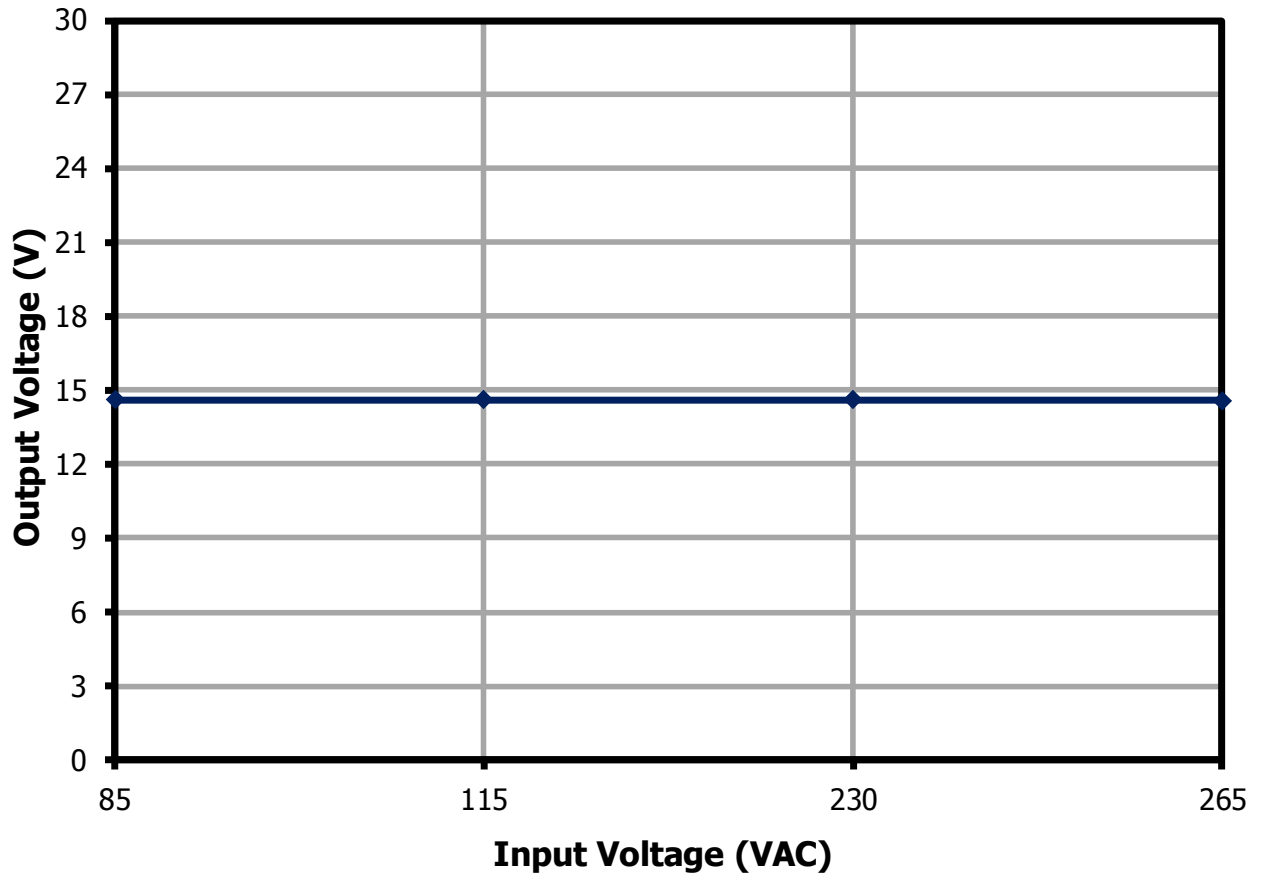
Figure 26 – Output Voltage vs. Input Line Voltage for 15 V Output, Room Temperature.
