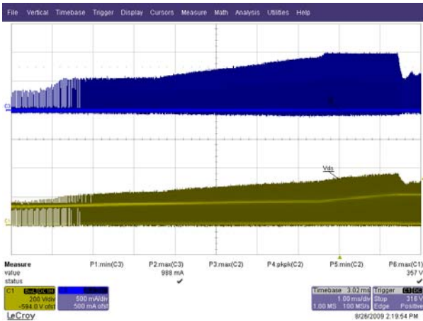
Figure 19 – 85 VAC Input and Maximum Load. Upper: I_{DRAIN} , 0.5 A / div. Lower: V_{DRAIN} , 100 V & 1 ms / div.
