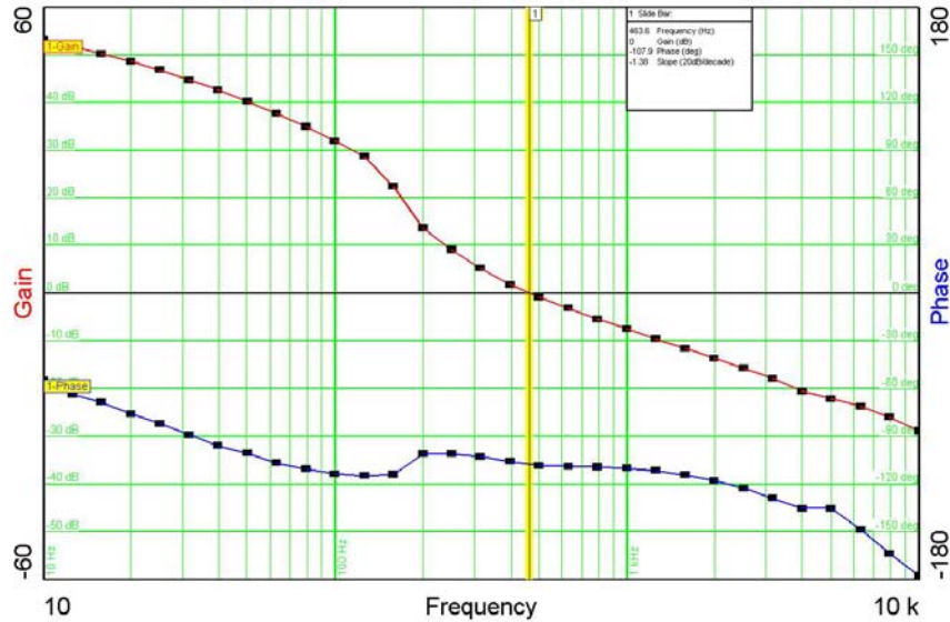
Figure 29 – Gain-Phase Plot, 180 VAC, Maximum Steady State Load. Vertical Scale: Gain = 10 dB / div, Phase = 30 °/ div. Crossover Frequency = 463 Hz Phase Margin = 72.1°
