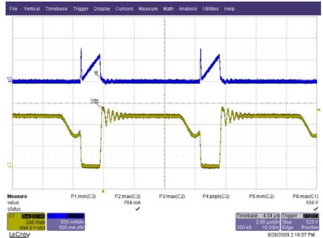
Figure 16 – 265 VAC, Full Load. Upper: I_{DRAIN} , 0.5 A / div. Lower: V_{DRAIN} , 200 V / div.
