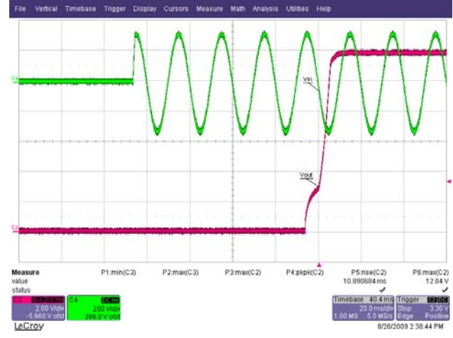
Figure 18 – Start-up Profile, 230 VAC, 20 ms / div. Upper: V_{IN} , 200 V / div. Lower: V_{OUT} , 2 V / div.
