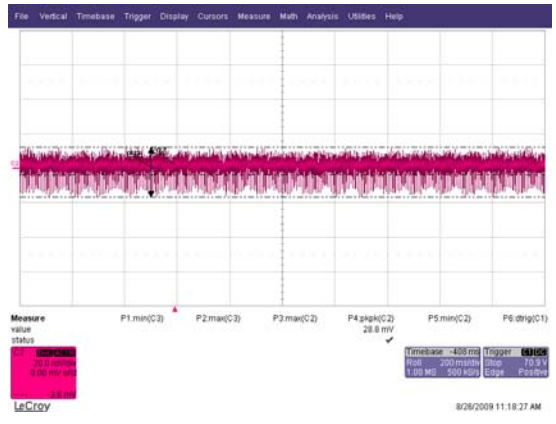
Figure 26 – 5 V Ripple [29 mV PP ], 115 VAC, Full Load. 200 ms, 20 mV / div.
