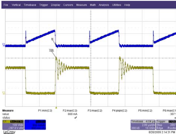
Figure 15 – 85 VAC, Full Load. Upper: I_{DRAIN} , 0.5 A / div. Lower: V_{DRAIN} , 100 V, 2 μs / div.
