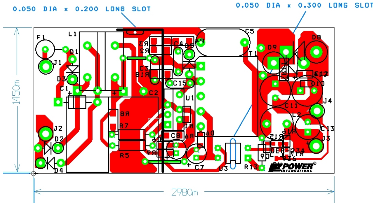
Figure 3 – Printed Circuit Layout (1450 mils x 2980 mils).
