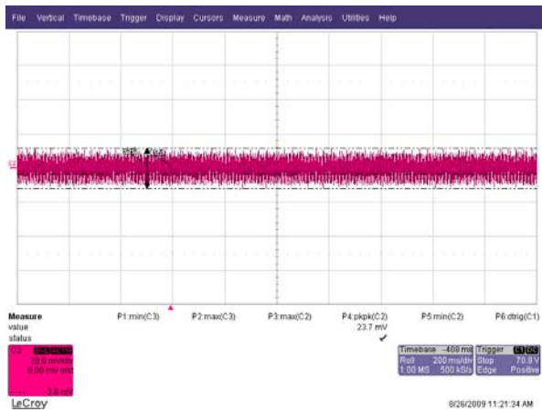
Figure 28 – Ripple [24 mV PP ], 265 VAC, Full Load. 200 ms, 20 mV / div.
