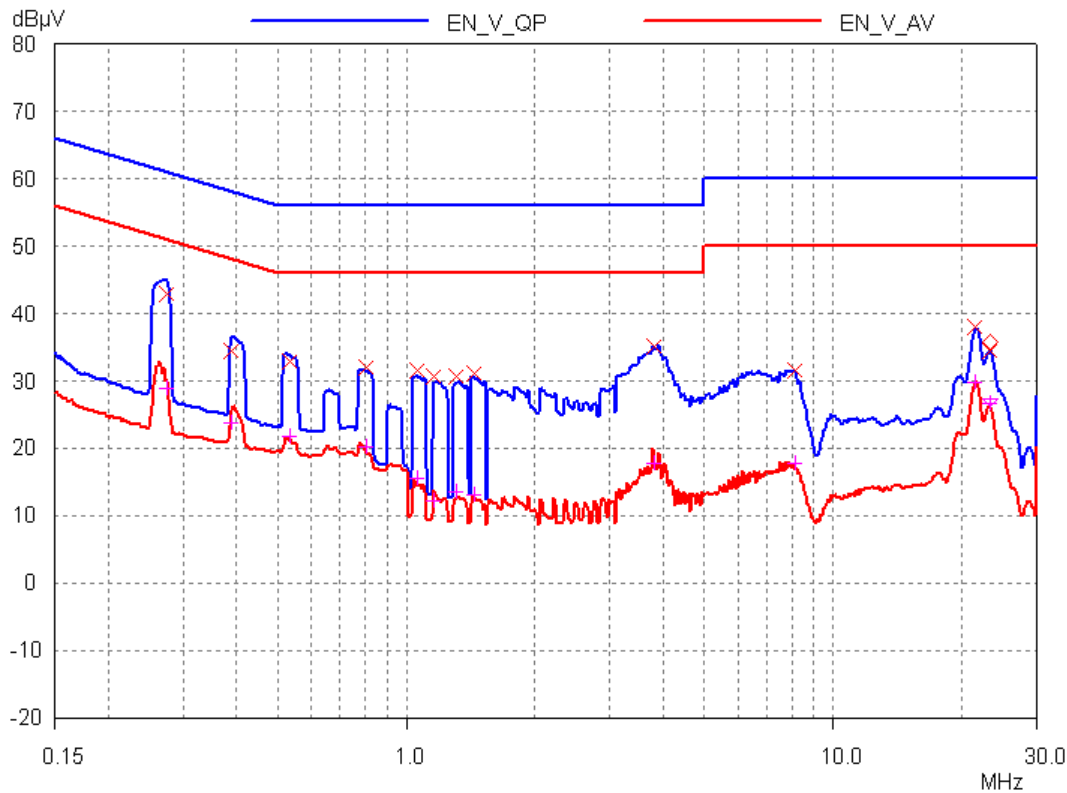
Figure 31 – Conducted EMI, Maximum Steady State Load, 115 VAC, 60 Hz, and EN5022 B Limits. Output Not Connected to PE (Floating).
