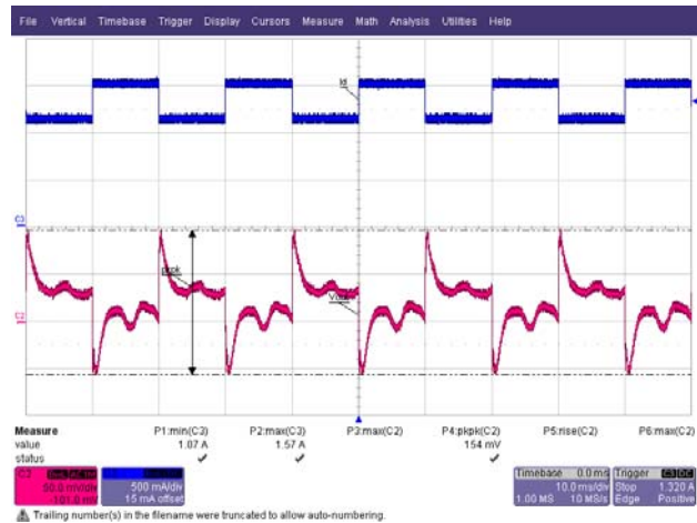
Figure 22 – Transient Response, 230 VAC, 75-100-75% Load Step. Upper: Load Current, 1 A / div. Lower: Output Voltage 50 mV, 2 ms / div.
