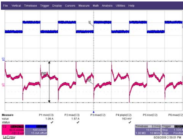
Figure 21 – Transient Response, 115 VAC, 75-100-75% Load Step. Top: Load Current, 1 A / div. Lower: Output Voltage 50 mV, 500 \mu s / div.
