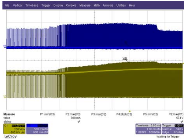
Figure 20 – 265 VAC Input and Maximum Load. Upper: I_{DRAIN} , 0.5 A / div. Lower: V_{DRAIN} , 200 V & 1 ms / div.
