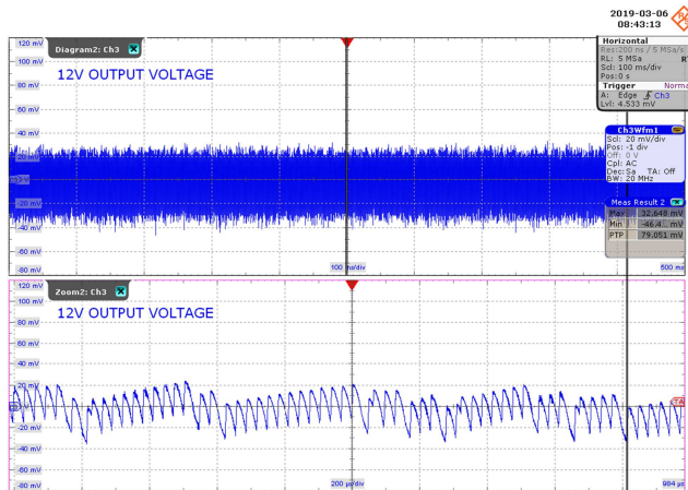
Figure 31 – Output Voltage Ripple Waveforms. 85 VAC, 120 mA Output. 20 mV, 100 ms / div.; 200 \mu\text{s} / div. V_{\text{PK-PK}} : 79.051 mV.
