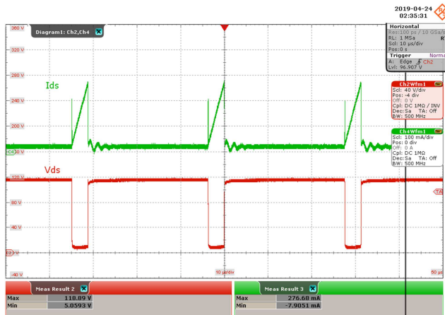
Figure 14 – Drain Voltage and Current Waveforms. 85 VAC, 120 mA Output. Upper: I_{DRAIN} , 100 mA / div. Lower: V_{DRAIN} , 40 V, 10 \mu s / div. I_{MAX} = 276.7 mA, V_{MAX} = 118.9 V.
