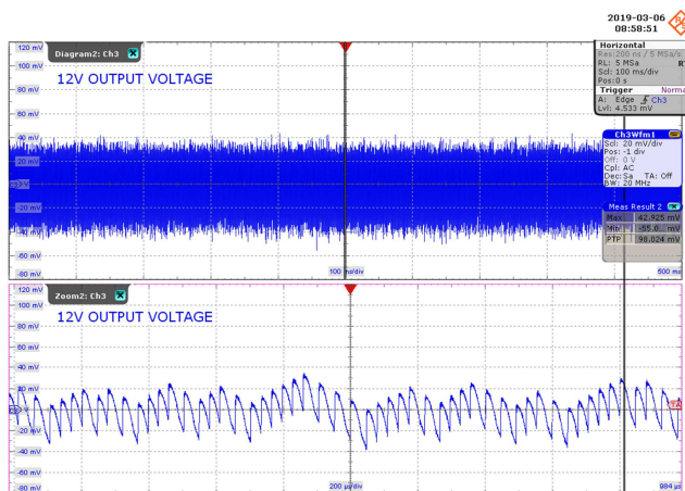
Figure 33 – Output Voltage Ripple Waveforms. 265 VAC, 120 mA Output. 20 mV, 100 ms / div.; 200 \mu\text{s} / div. V_{\text{PK-PK}} : 98.024 mV.
