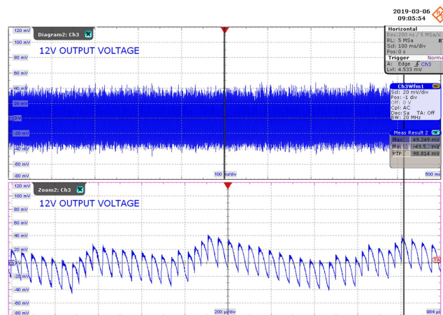
Figure 34 – Output Voltage Ripple Waveforms. 440VAC, 120 mA Output. 20 mV, 100 ms / div.; 200 \mu\text{s} / div. V_{\text{PK-PK}} : 98.814 mV.
