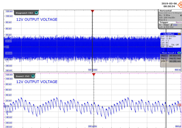
Figure 32 – Output Voltage Ripple Waveforms. 230VAC, 120 mA Output. 20 mV, 100 ms / div.; 200 \mu\text{s} / div. V_{\text{PK-PK}} : 93.281 mV.
