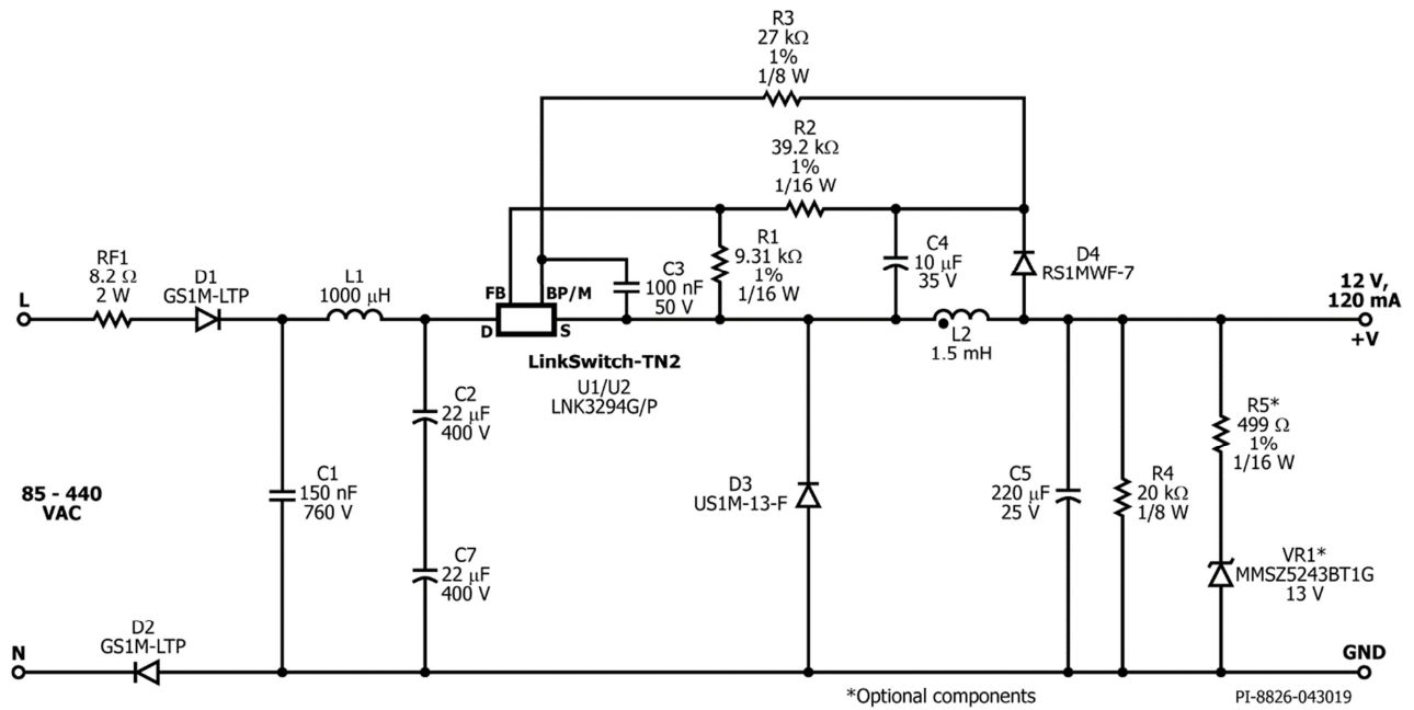
Figure 3 – Schematic.
