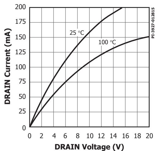
Figure 17. Output Characteristics.
