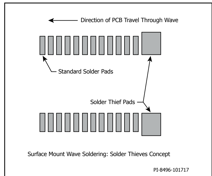
Figure 5. Solder Thieves Concept.
