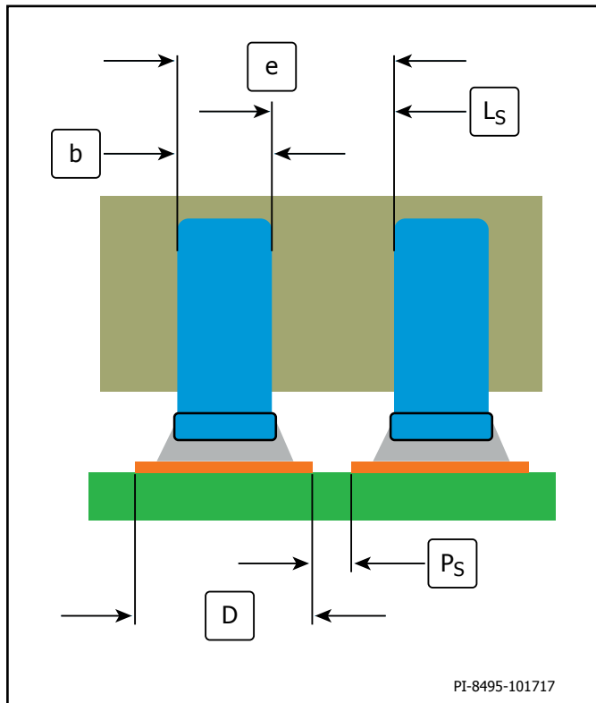
Figure 4. Solder Pad Spacing.
