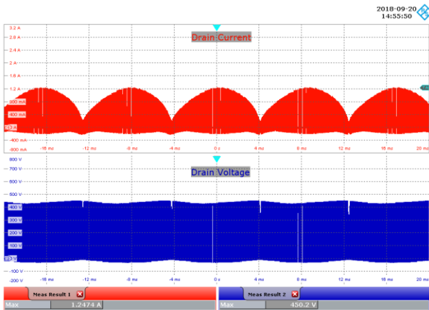
Figure 73 – 277 VAC, 48 V LED Load. Upper: I_{DRAIN} , 400 mA / div. Lower: V_{DRAIN} , 100 V / div., 4 ms / div.
