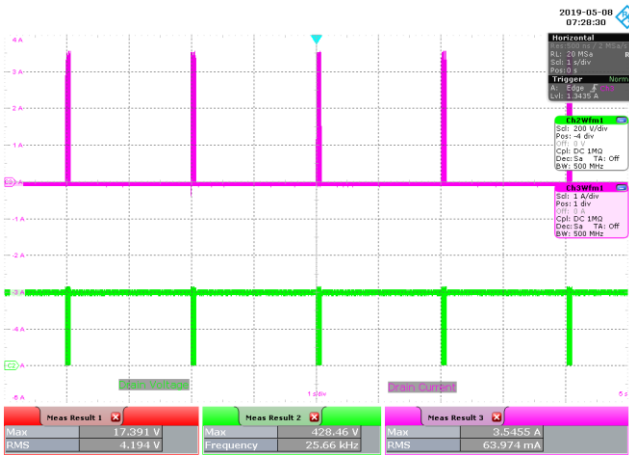
Figure 97 – 277 VAC, Output Shorted. Upper: I_{DRAIN} , 1 A / div. Lower: V_{DRAIN} , 200 V / div., 1 s / div.
