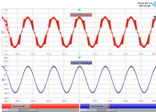
Figure 47 – 100 VAC, 48 V LED Load. Upper: I_{IN} , 500 mA / div. Lower: V_{IN} , 50 V / div., 10 ms / div.
