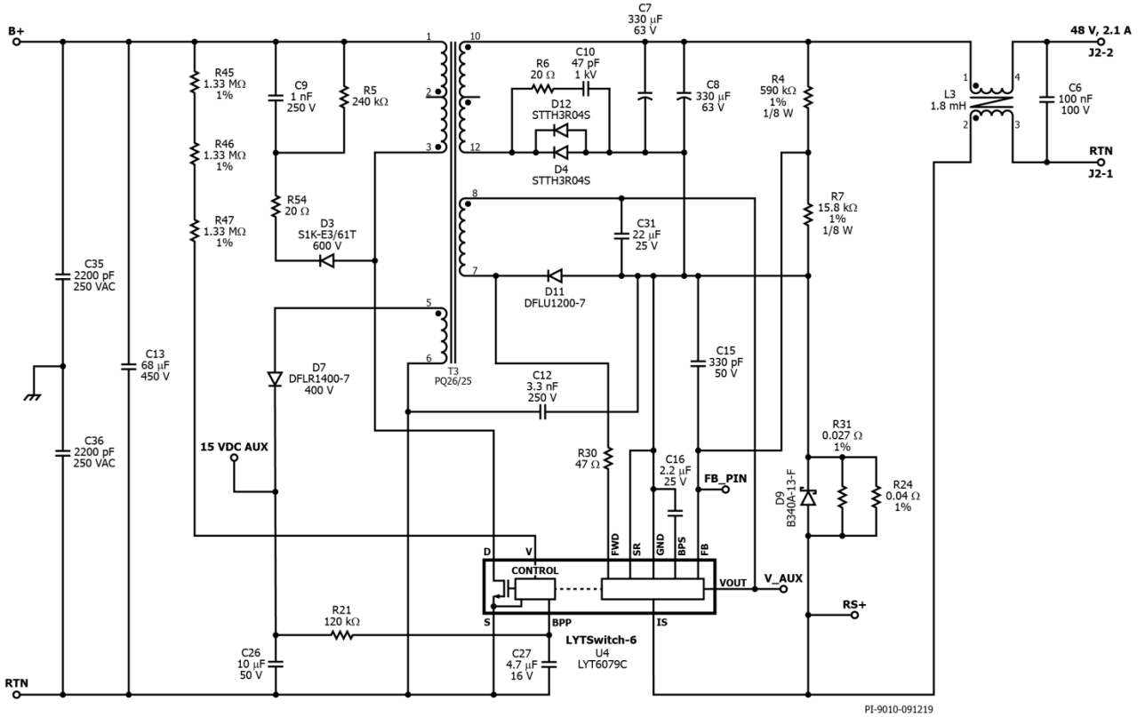
Figure 10 – Schematic, Power Section.
