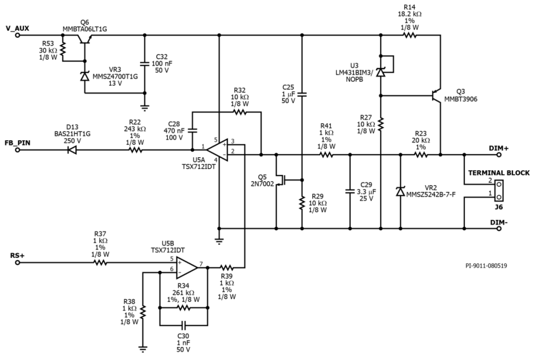
Figure 11 – Schematic, Dimming Section.
